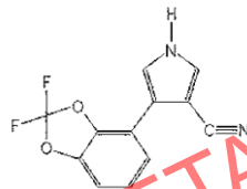
Fludioxonil
