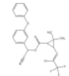
Lambda-cyhalothrin
