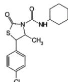
Hexythiazox
