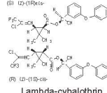
Lambda-cyhalothrin
