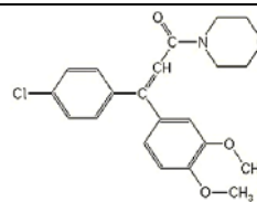
Dimethomorph
