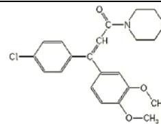
Dimethomorph
